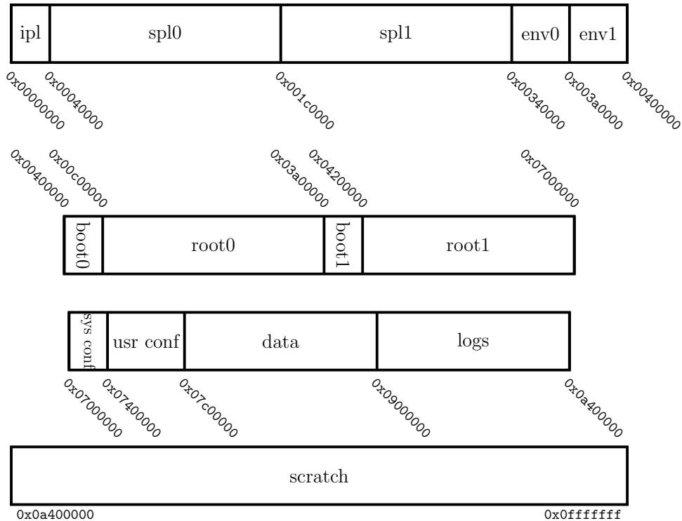
Figure 4: NAND layout
